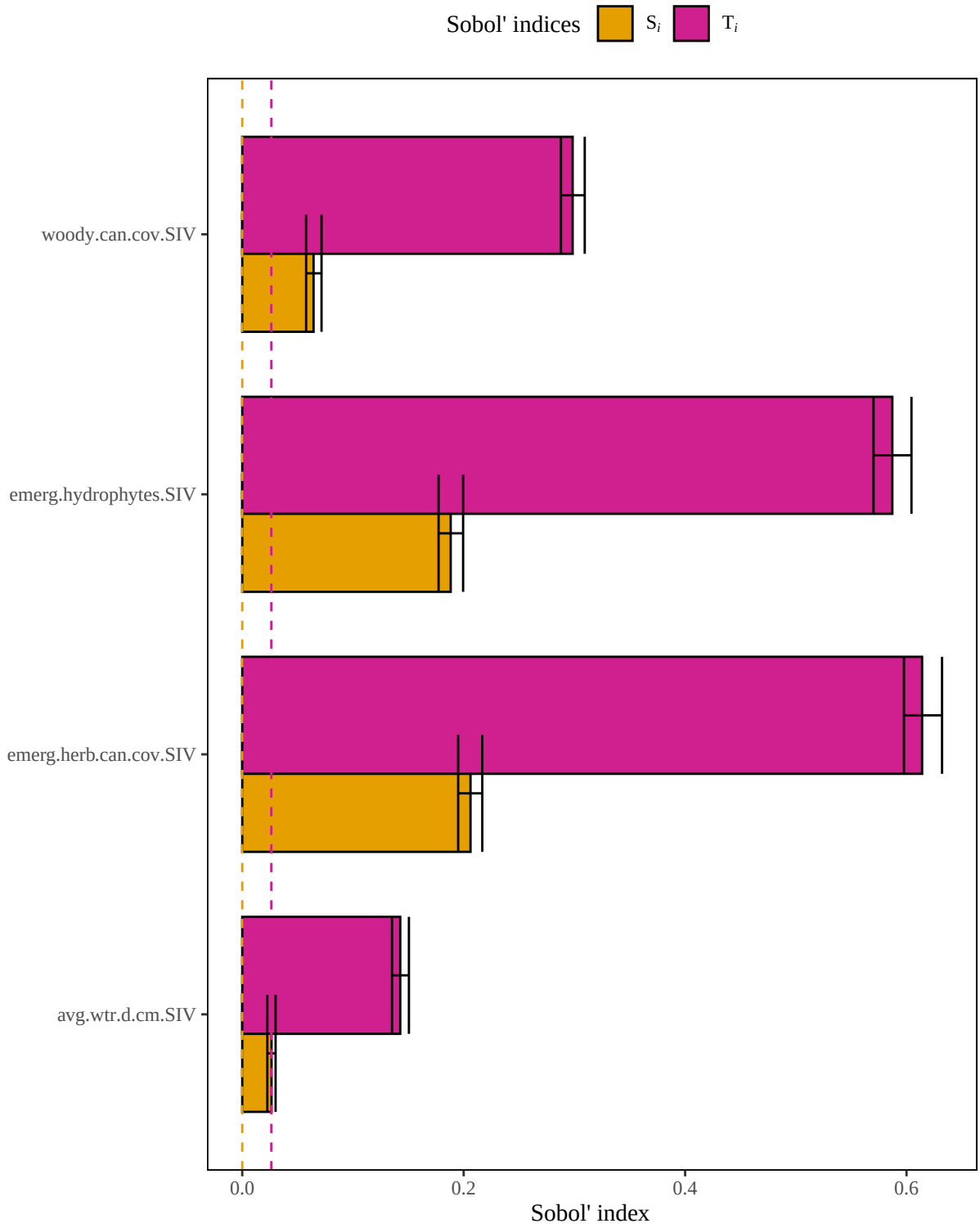
Figure 7. Results of a sensitivity analysis for the marshwren model based on a multiplicative mean structure. Dashed lines represent baseline numerical approximation error for S_i and T_i ( i.e. , dummy variables).
